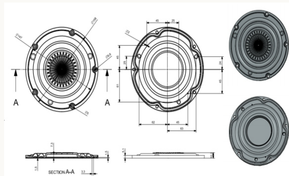
LENS DIMENSION
